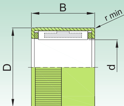
HF..R / HF..KFR
