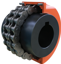
BS Coupling
